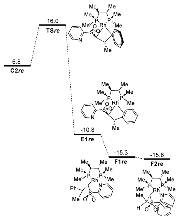
FIGURE 3. Energy profile for the insertion step through the \beta -re face to give the major enantiomer ( S )-4g. Relative energies (kcal mol -1 ) evaluated with respect to RhPh(H 2 O)(modL*)+3g-H 2 O. ZPE correction included.
