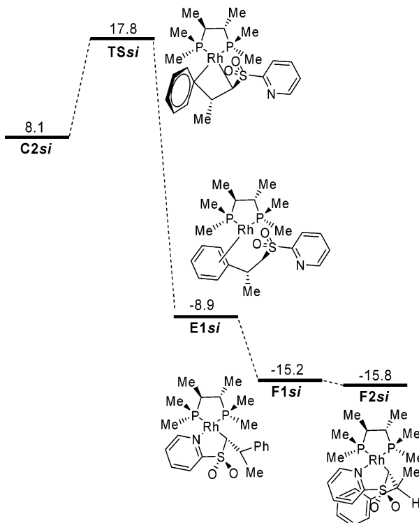
FIGURE 4. Energy profile for the insertion step through the \beta -si face to give the minor enantiomer ( R )-4g. Relative energies (kcal mol -1 ) evaluated with respect to RhPh(H 2 O)(modL*)+3g-H 2 O. ZPE correction included.
