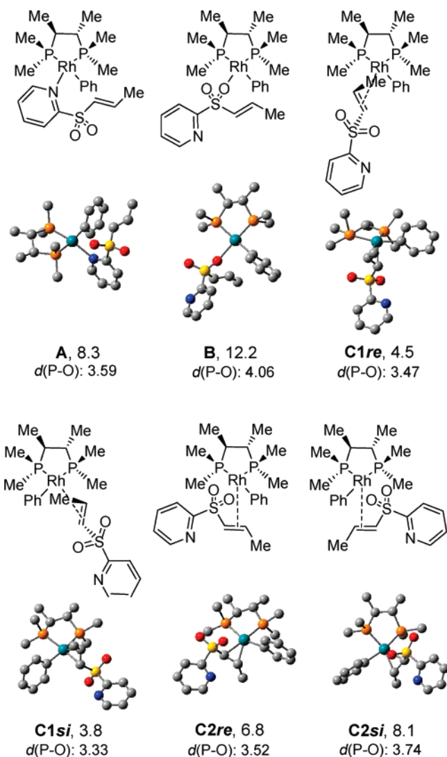
FIGURE 2. Relative energies (kcal mol -1 ) evaluated with respect to RhPh(H 2 O)(modL*)+3g-H 2 O. ZPE correction included. The closest P–O distances (Å) are also indicated. Hydrogen atoms have been omitted for clarity.
