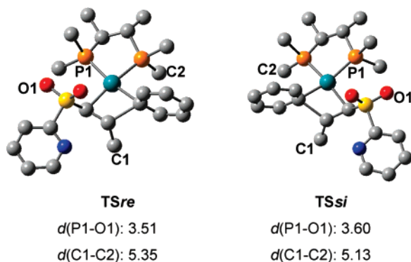
FIGURE 5. Molecular structures of transition states TSre and TSsi . Distances (Å) between selected atoms are also indicated. Hydrogen atoms have been omitted for clarity.
